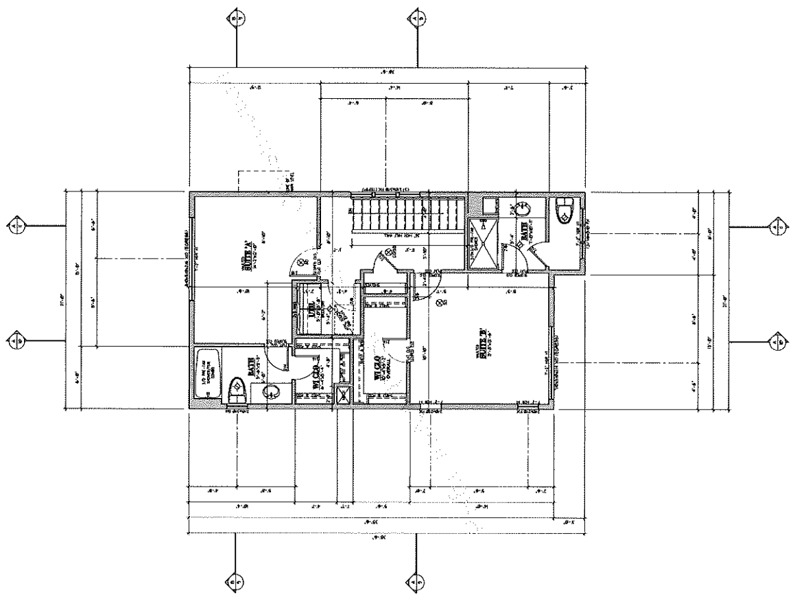
UPPER LEVEL FLOOR PLAN SCALE: 1/8" = 1'-0" 1/8" = 1'-0"
